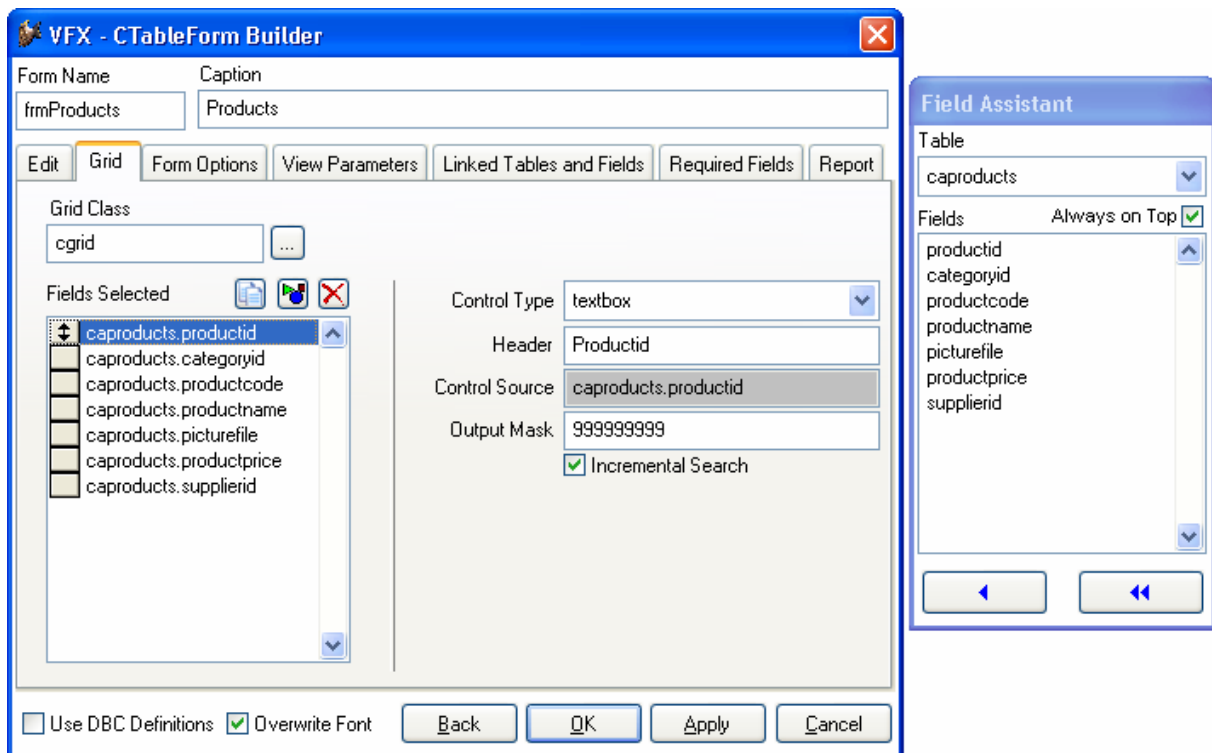
VFX – CTableForm Builder, Grid Page
