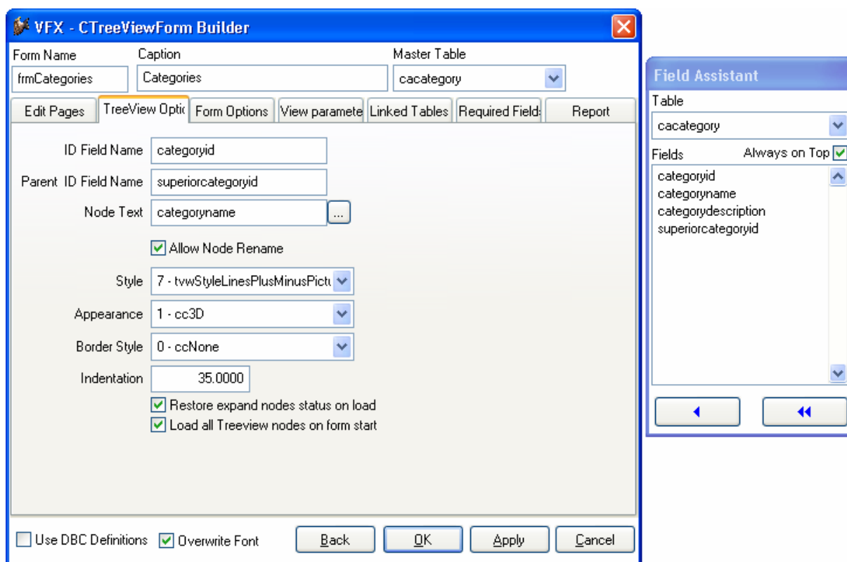
VFX – CTreeViewForm Builder
