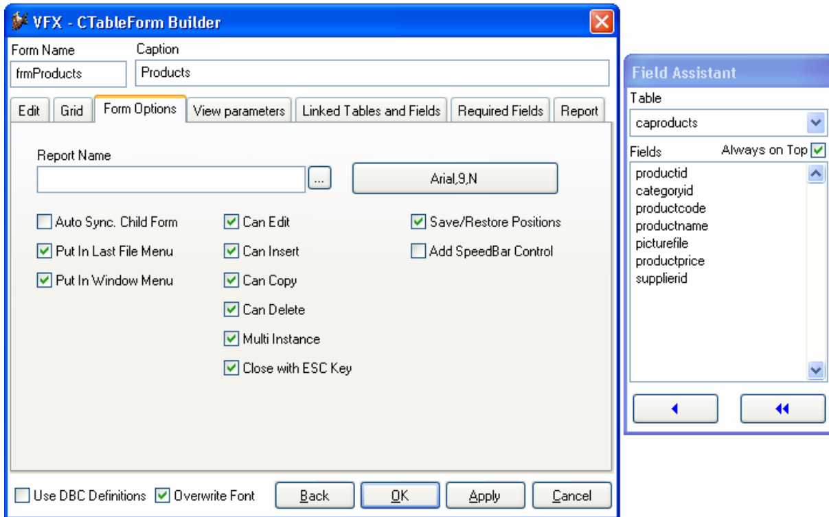
VFX – CTableForm Builder, Form Options Page
