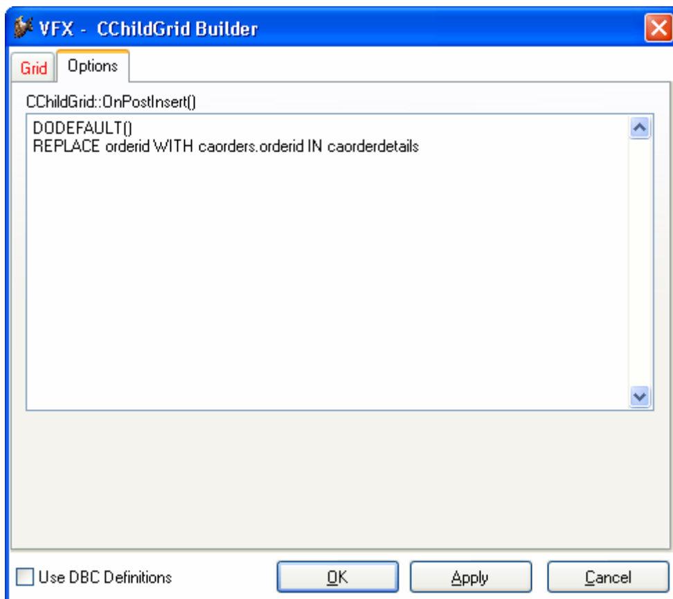
VFX – CChildGrid Builder, Options Page
