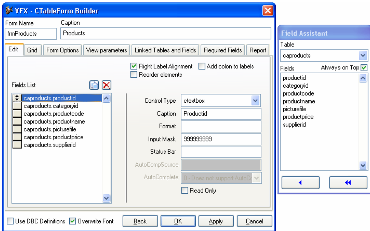
VFX – CTableForm Builder, Edit Page
