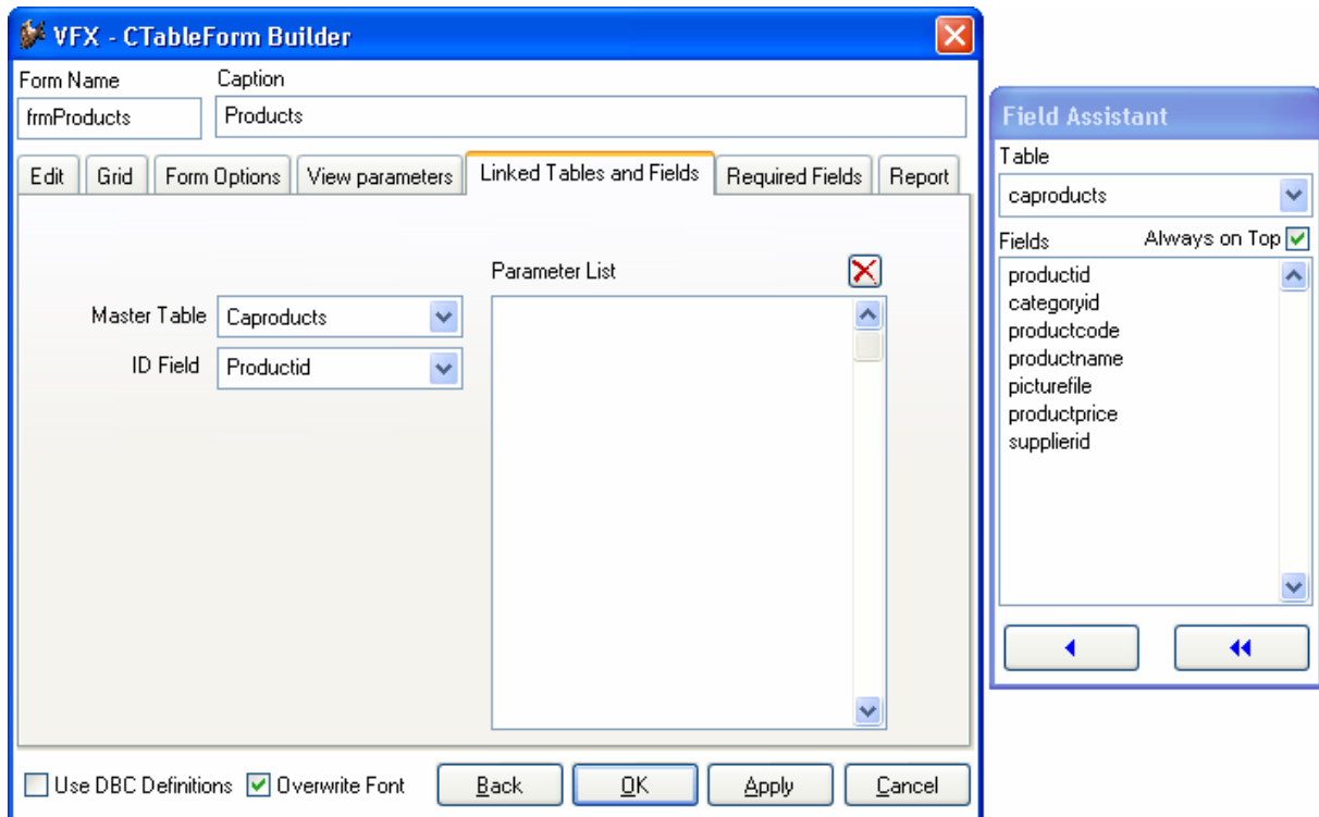
VFX – CTableForm Builder, Linked Tables and Fields Page
