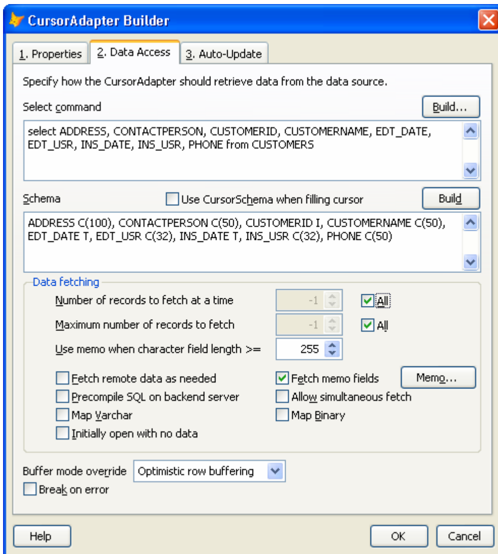
VFP CursorAdapter Builder, Data Access
