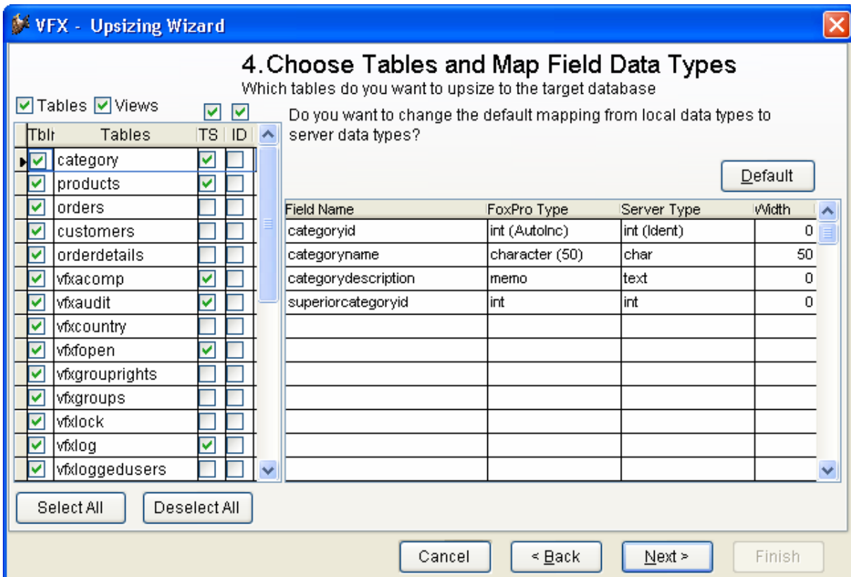
VFX – Upsizing Wizard, Choose Tables and Map Field Data Types
