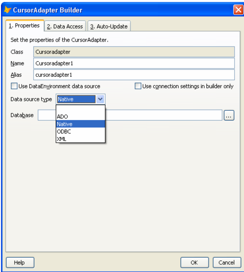
VFP CursorAdapter Builder, Properties
